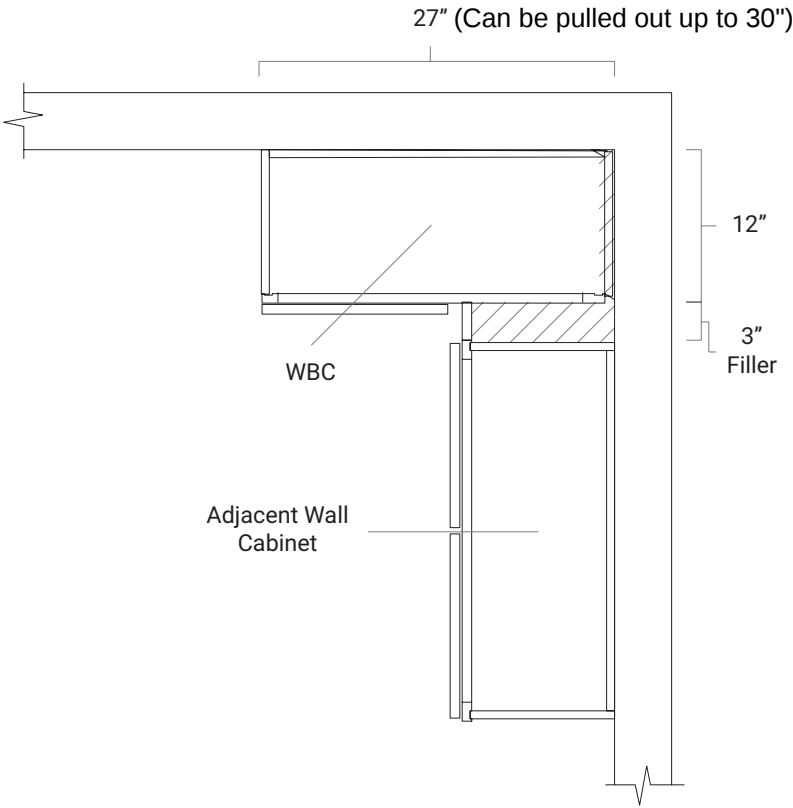
INSTALLATION DIAGRAM
