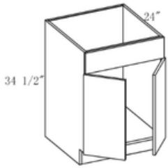
Sink Base Cabinet 2 doors 1 fake drawer
