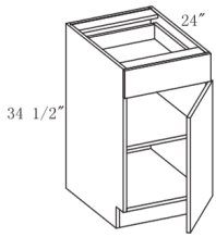
Base Cabinet 1 door 1 Drawer, 1 Shelf
