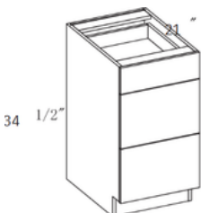
Vanity Drawer Base Cabinet 3 drawers: 6" 12" 12"
