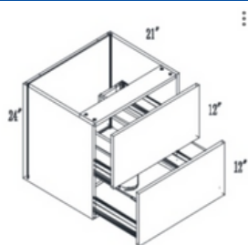
Vanity Drawer Base Cabinet 2 drawers: 12" 12"
