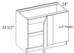
Base Blind Corner Cabinet
