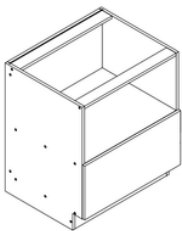
Microwave Base Cabinet with 1 drawer 12"
