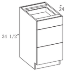
Base Cabinet with 3 Drawers: 6", 12", 12"
