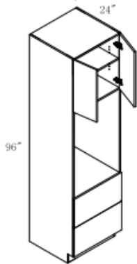
Microwave + Oven Cabinet 2 doors, 2 drawers, 1 shelf
