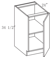
Base Cabinet 1 Full Height Door No Drawer, 1 Shelf
